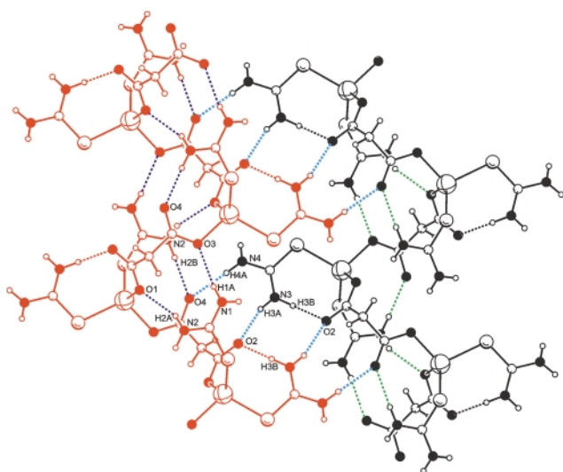
Fig. 5 Hydrogen bonding in compound 3 . The intra-chain hydrogen bonds are depicted in blue or green and have distances (Å) and angles (°) of N(2)⋯O(4) 2.864(3), H(2B)⋯O(4) 1.99(2), N(2)–H(2B)⋯O(4) 172(2); N(1)⋯O(3) 2.923(3), H(1A)⋯O(3) 2.08(2), N(1)–H(1A)⋯O(3) 167(2); and N(2)⋯O(1) 2.905(3), H(2A)⋯O(1) 2.09(2), N(2)–H(2A)⋯O(1) 154(2). The inter-chain hydrogen bonds are depicted in cyan and have distances (Å) and angles (°) of N(3)⋯O(2) 2.840(3), H(3A)⋯O(2) 2.02(2), N(3)–H(3A)⋯O(2) 156(2); and N(4)⋯O(4) 2.946(3), H(4A)⋯O(4) 2.06(2), N(4)–H(4A)⋯O(4) 173(3).
