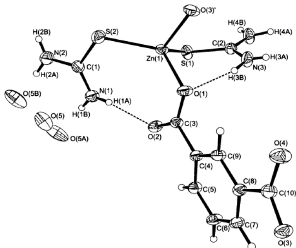
Fig. 6 The zinc co-ordination sphere in compound 4 . The hydrogen bond distances (Å) and angles (°) are N(1)⋯O(2) 2.817(4), H(1A)⋯O(2) 2.06(4), N(1)–H(1A)⋯O(2) 167(4); and N(3)⋯O(1) 3.079(4), H(3B)⋯O(1) 2.20(5), N(3)–H(3B)⋯O(1) 161(4).
