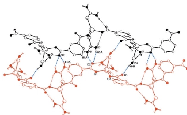
Fig. 7 Inter-chain hydrogen bonding in compound 4 . The hydrogen bond distances (Å) and angles (°) are N(3)⋯O(2) 2.938(4), H(3A)⋯O(2) 2.33(4), N(3)–H(3A)⋯O(2) 151(5); N(4)⋯O(2) 2.860(4), H(4A)⋯O(2) 2.05(5), N(4)–H(4A)⋯O(2) 156(4); and N(4)⋯O(4) 2.840(4), H(4B)⋯O(4) 2.08(5), N(4)–H(4B)⋯O(4) 159(4).
